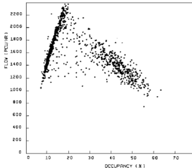
Fig. 2: Time averaged flow density relationship
