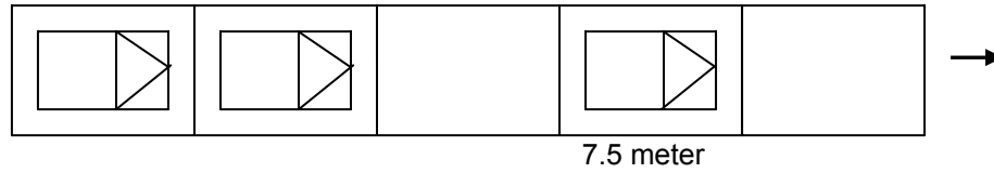
Fig. 3: A typical configuration of Nagel-Schreckenberg (1992) model
