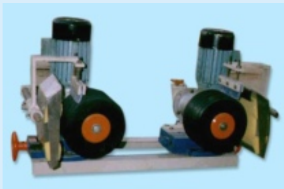
Water Scraping Device Suitable for removing excess glaze from tile sides
