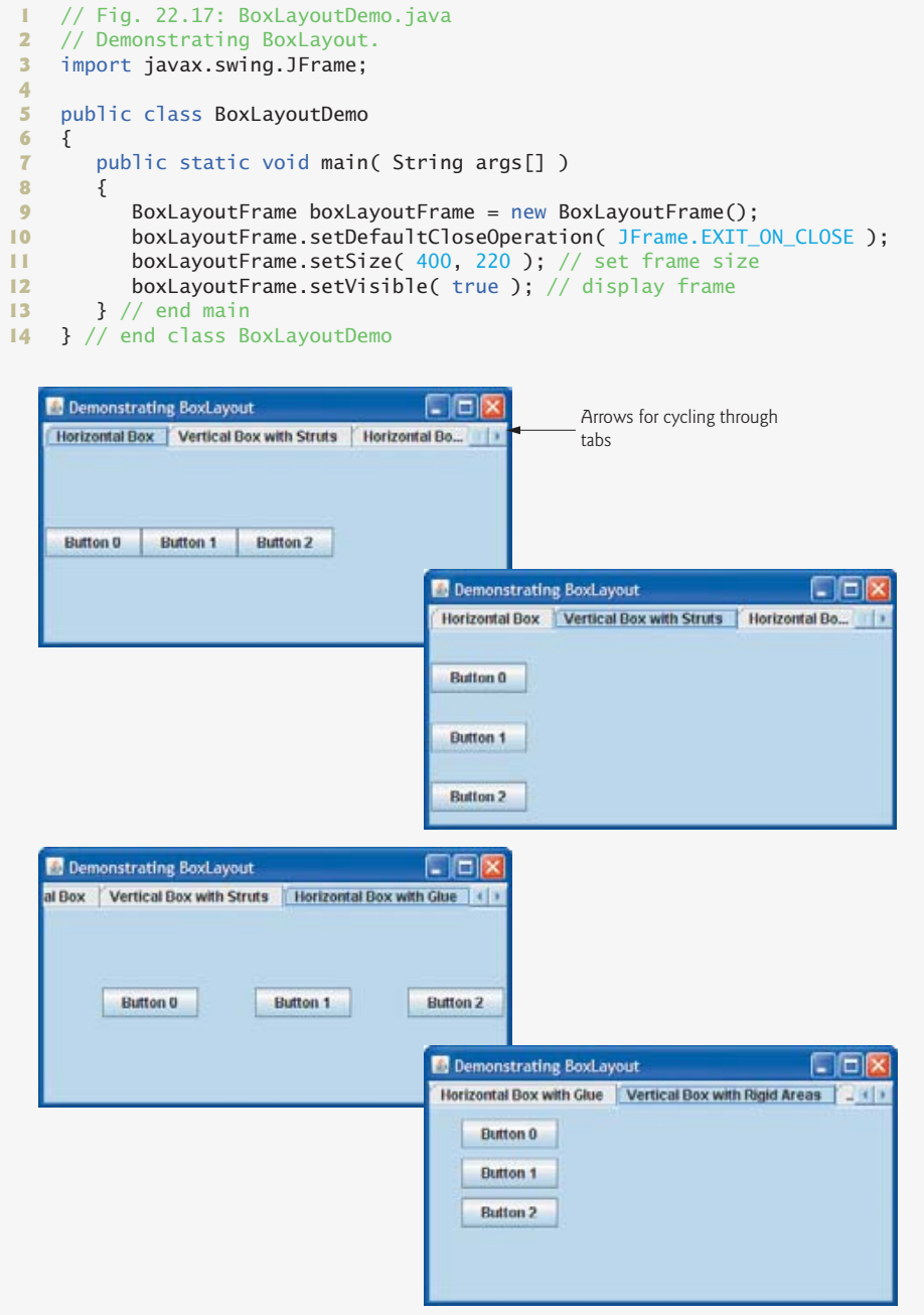
Fig. 22.17 | Test class for BoxLayoutFrame. (Part 1 of 2.)
