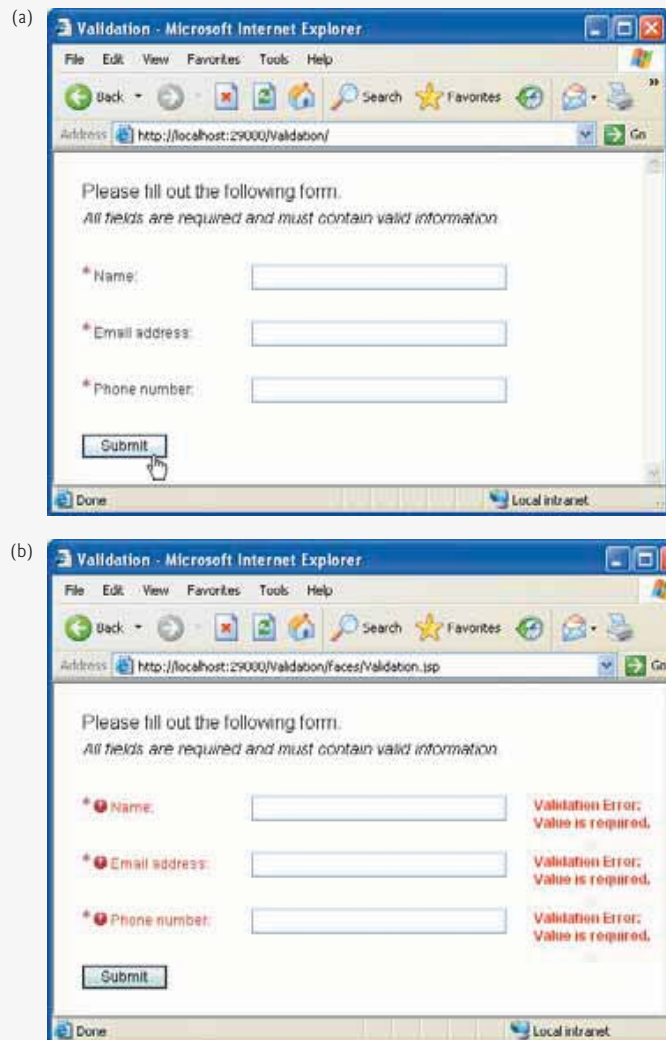
Fig. 26.18 | JSP that demonstrates validation of user input. (Part 3 of 4.)
