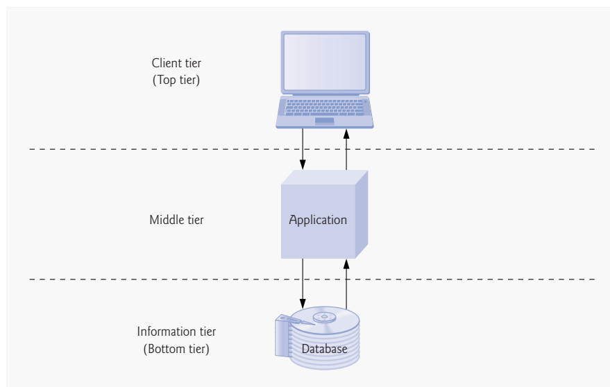
Fig. P.8 | Three-tier application model.
