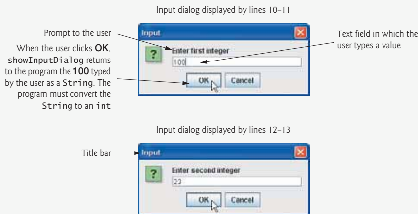
Fig. 11.2 | Addition program that uses JOptionPane for input and output. (Part I of 2.)
