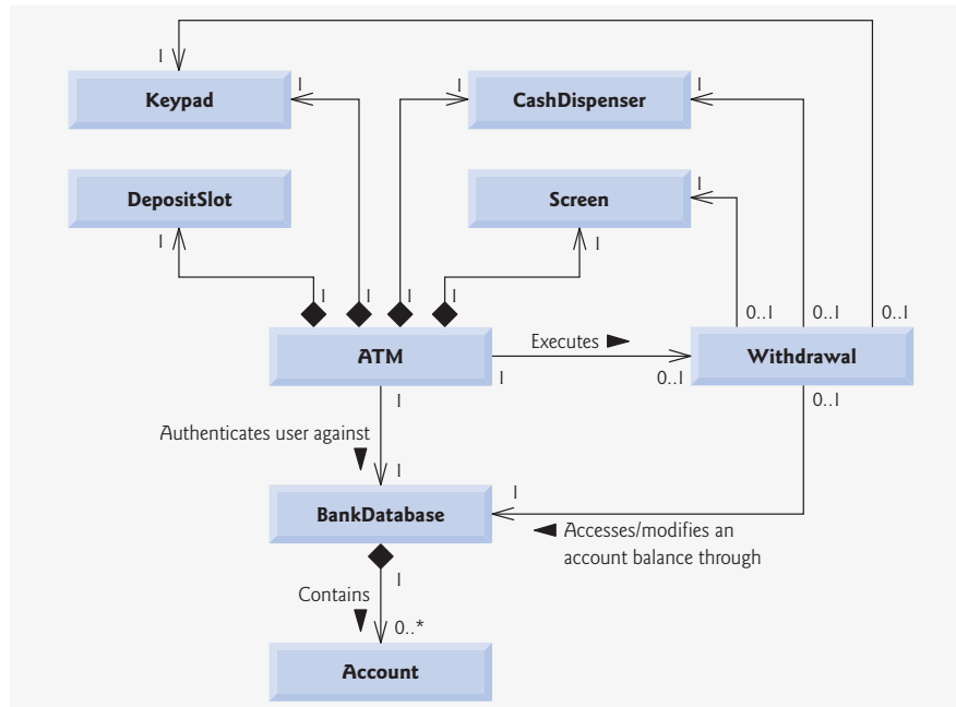
Fig. 8.25 | Class diagram with navigability arrows.
