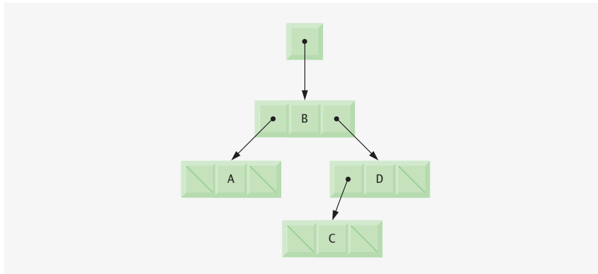
Fig. 17.15 | Binary tree graphical representation.
