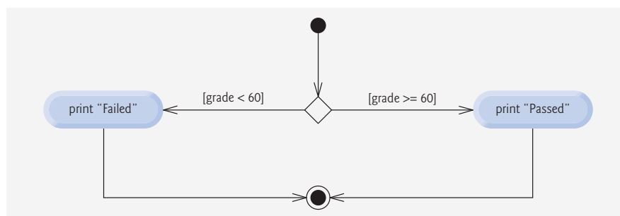
Fig. 4.3 | if...else double-selection statement UML activity diagram.
