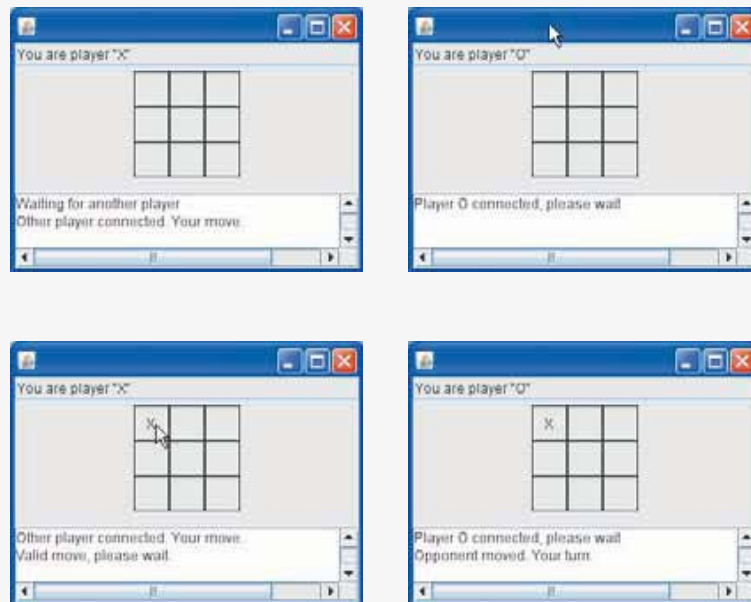
Fig. 24.17 | Sample outputs from the client/server Tic-Tac-Toe program. (Part I of 2.)
