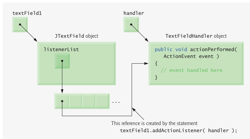
Fig. 11.13 | Event registration for TextField textField1 .
