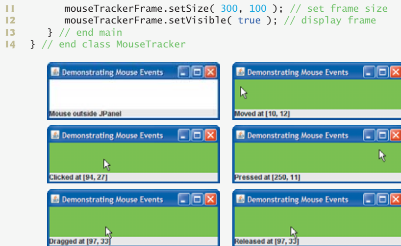
Fig. 11.29 | Test class for MouseTrackerFrame . (Part 2 of 2.)
