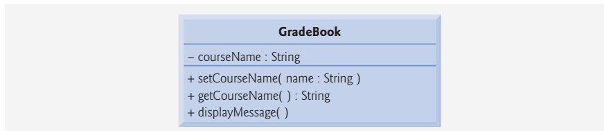
Fig. 3.9 | UML class diagram indicating that class GradeBook has a courseName attribute of UML type String and three operations— setCourseName (with a name parameter of UML type String ), getCourseName (which returns UML type String ) and displayMessage .
