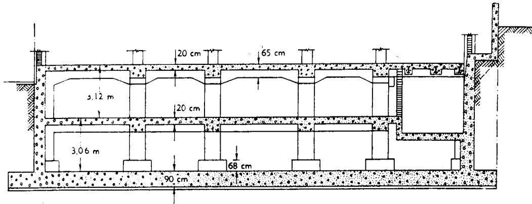
Figura 3.8: Radier
