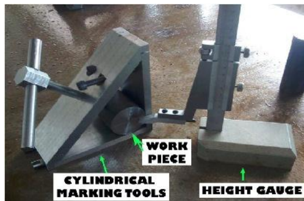
Figure 2 Work piece preparations on surface table.
