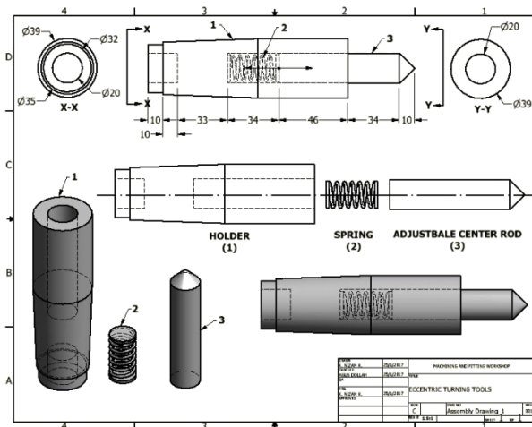
Figure 3 Assembled Diagram of Eccentric Turning Tools, ETT
