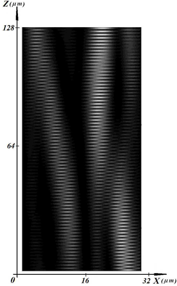
FIG. 1: Gray scale intensity plot for a small volume of a speckle pattern inside PC-mirror in (X, Z) -plane ( Y = 23\mu m ). The mean transverse size of a speckle is D \sim 8\mu m . The mean longitudinal length of a speckle entity is of the order of the Rayleigh range L_R \approx D^2/\lambda for \lambda \sim 1\mu m . The size of the volume is 32\mu m in transverse (X, Y) directions and 128\mu m in longitudinal (Z) direction. The step of longitudinal modulation \cos((k_p + k_s)z \pm 2\phi) induced by the interference of counter-propagating pump and Stokes waves is enlarged here 8 times for visualization purposes. The characteristic \pi -phase-jump is clearly visible in between adjacent Bragg's \cos -modulated roll patterns.
