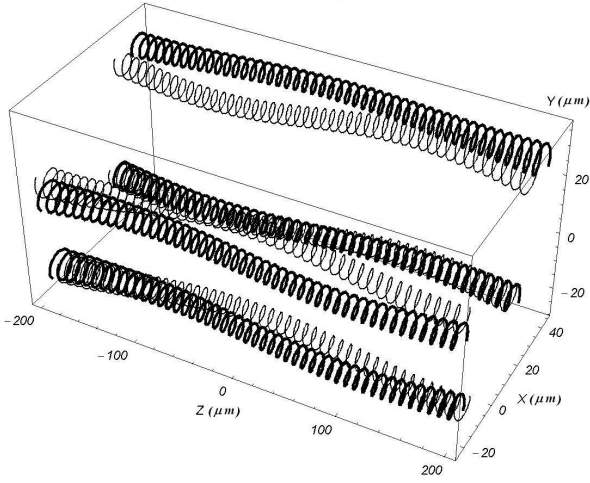
FIG. 2: The plot of the light intensity maxima at a given moment t in a small volume inside the PC-mirror. The four pairs of spiral interference patterns with opposite handedness are located randomly in space. Their diameters and directions are changed smoothly due to diffraction. The step of longitudinal modulation \cos((k_p + k_s)z \pm 2\phi) is enlarged here 16 times.
