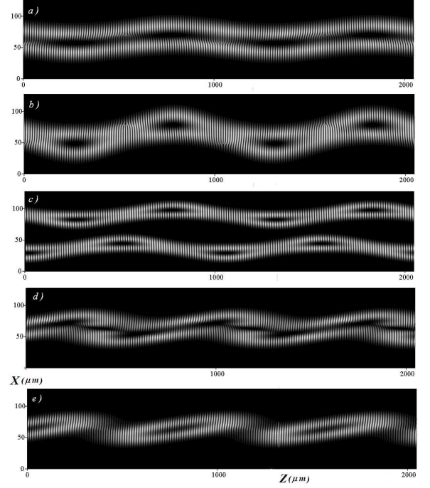
FIG. 3: Gray scale intensity plot for the variational ansatz (7) substituted in (5). The 128 \times 2048 points arrays are used for the intensity distributions (5) in X \times Z planes at fixed Y=64 . The single sinusoidally modulated LG_0^1 vortex line (see eq. (7)) is shown for M = 0.1 \cdot D (a) and M = D (b). Two LG_0^1 distant vortex lines LG_0^1 (c) with parallel (d) opposite (e) topological charges \pm\ell constitute the rope when the distance between them is reduced to zero(d,e). The step of longitudinal modulation is enlarged here 32 times.
