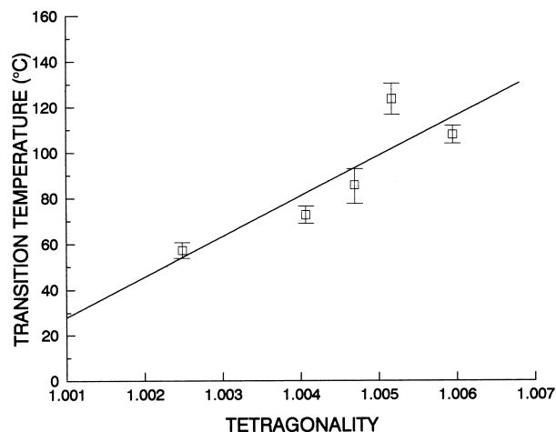
Fig. 6. Transition temperature against tetragonality for \text{Ba}_{1-x}\text{Sr}_x\text{TiO}_3 .
