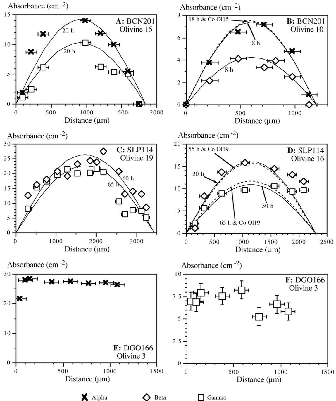
Fig. 2. Polarized infrared absorption intensities measured as area beneath the OH peaks across olivine grains from edge to edge. Analyses were made with an aperture of 150 \mu\text{m} (the "x error bar"), with the uncertainty on the absorbance for these olivines being 0.2 \text{cm}^{-2} (about the size of the symbols except for DGO166 Olivine 3 gamma, panel F). The absorption is highest at the center of the olivines of BCN201 and lowest to absent at their edges. These typical diffusion profiles are interpreted to illustrate the loss of hydrogen undergone by the olivines during transport of the xenolith from the upper mantle to the surface by its host mafic alkalic magma. Crystals that do not show symmetrical patterns of rimward hydrogen loss (DGO166 Olivine 3, panels E and F, and one side of SLP114 Olivine 16, panel D) may not be true intact grain boundaries, but instead broken crystal edges generated when the xenoliths were disaggregated during sample preparation. In order to estimate the time of hydrogen loss, the profiles are modeled using Eq. (3) solved for the three terms of the series, a coefficient of hydrogen diffusion of 2.75 \times 10^{-12} \text{ m s}^{-1} , and a C_0 of 40% more than that measured in the center of the olivine (see text for details). For BCN201 Olivine 10 alpha (B), and for SLP114 Olivine 16 beta and gamma (D) the model was run two ways; one using the C_0 measured at the center of the olivine (8 h and 30 h, respectively, solid lines) and one using the C_0 measured at the center of a larger olivine from the same xenolith (18 h and 55–65 h, respectively, dashed lines).
