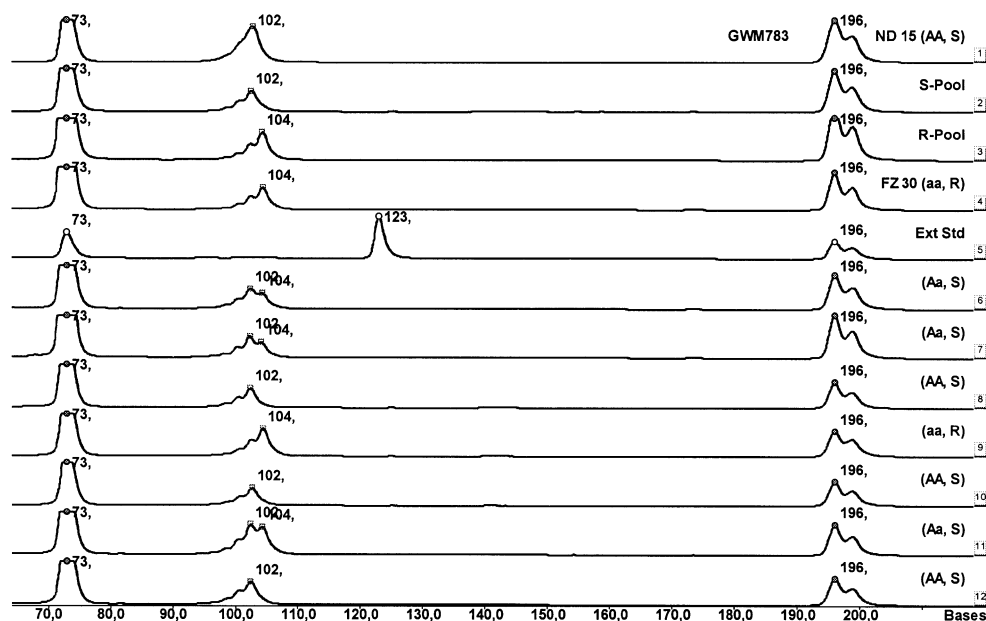
Fig. 1 Polymorphic microsatellite marker Xgwm783 analysed using Fragment Analyser version 1.02. The peaks represent fragments, whereas the horizontal scale indicates fragment sizes in base pairs calculated from internal standards (73 bp and 196 bp) and external standards (73 bp, 123 bp and 196 bp). The fragments 102 bp and 104 bp were produced by Nongda (ND) 15, S-Pool, R-Pool, Fuzhuang (FZ) 30 and some F_2 plants, respectively. Lanes 6, 7 and 11 were heterozygous susceptible plants; lanes 4, 10 and 12 were homozygous susceptible plants; lane 9 involved homozygous resistant plants
